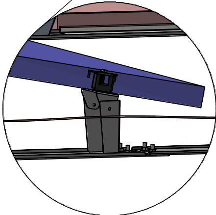
DETAIL B SCALE 1 : 7
